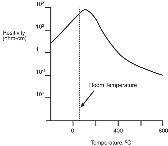
Figure 4-24. Resistivity of Silicon Doped with 10^{13} Carriers per Cubic Meter (32)
