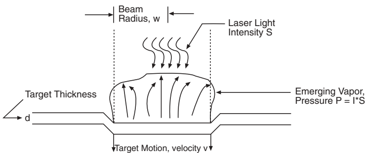
Figure 3-69. Mechanical Damage of a Target by a Laser
