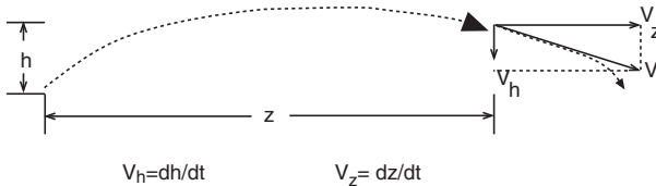
Figure 2-9. Projectile Distance and Velocity Coordinates
