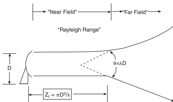
Figure 4-4. Rayleigh Range and Divergence
