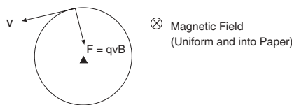
Figure 5-10. Motion of a Charged Particle in a Magnetic Field
