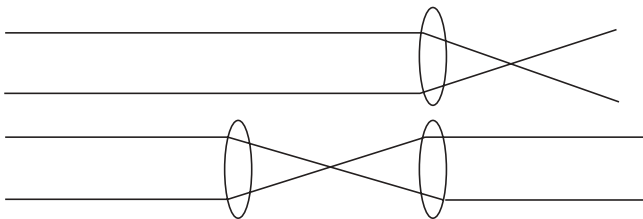
Figure 3-35. The Principle of Adaptive Optics
