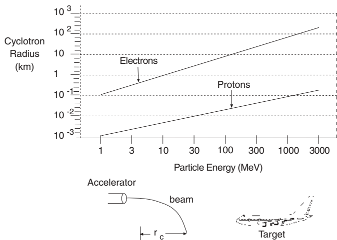
Figure 5-11. Cyclotron Radius vs Particle Energy for B = 0.5 Gauss
