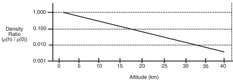
Figure 4-10. Relative Atmospheric Density vs Altitude
