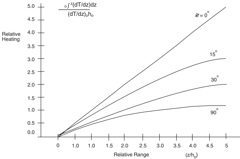
Figure 5-22. Relative Beam Heating vs Range and Elevation Angle
