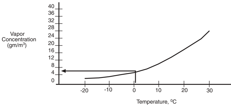
Figure 4-9. Concentration of Water Vapor vs Temperature at 100% Humidity
