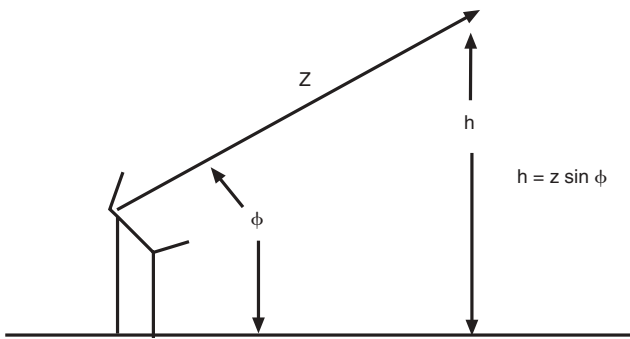
Figure 4-11. Beam Range and Altitude
