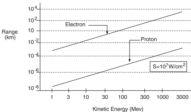
Figure 5-9. Doubling Distance for Electron and Proton Beams of Intensity 10^7 \text{ W/cm}^2
