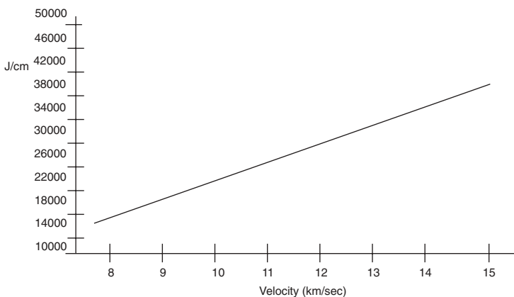
Figure 2-23. Kinetic Energy per Centimeter Penetrated vs Projectile Velocity
