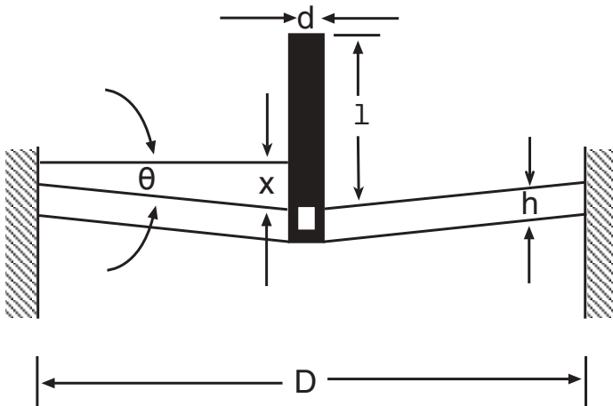
Figure 2-24. Penetration of a Plate by a Projectile
