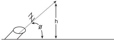
Figure 5-21. Charged Particle Beam Range and Altitude
