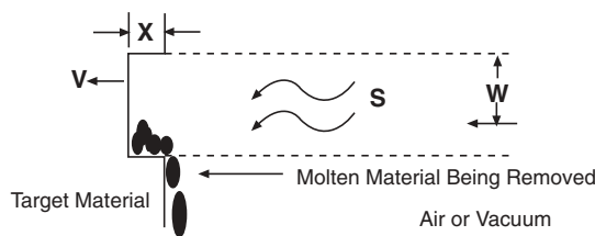
Figure 3-64. Hole Erosion with Molten Material Removed
